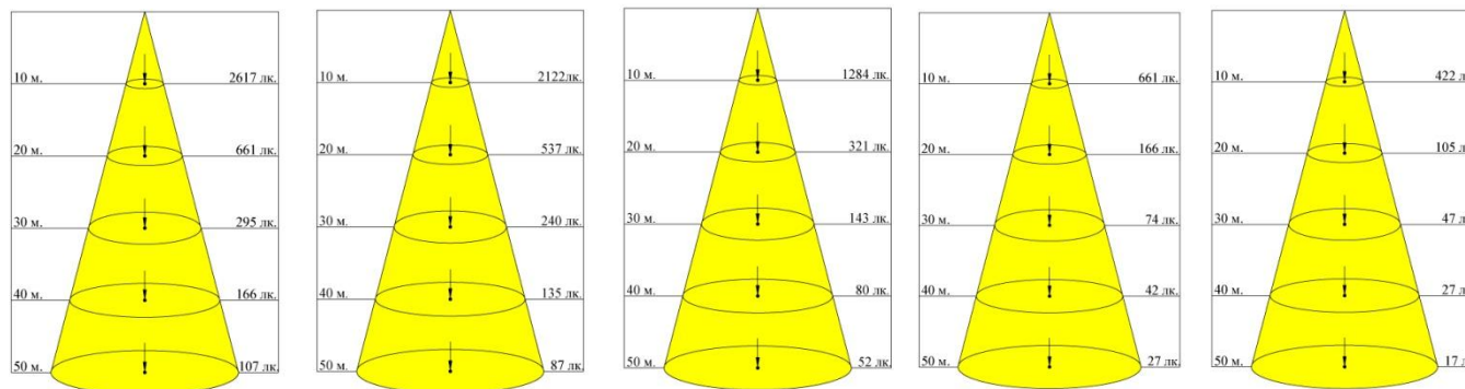
Geniled Solar 500-10°
